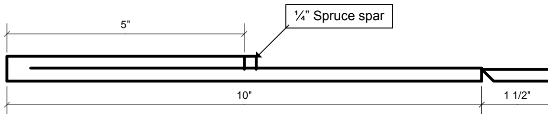
Option 1 wing – spar behind top surface
