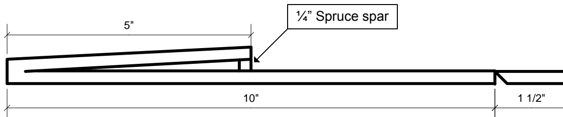
Option 2 wing – spar between surfaces
