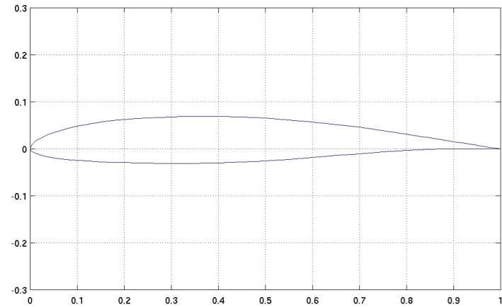
HQ 2.0/10 AIRFOIL
