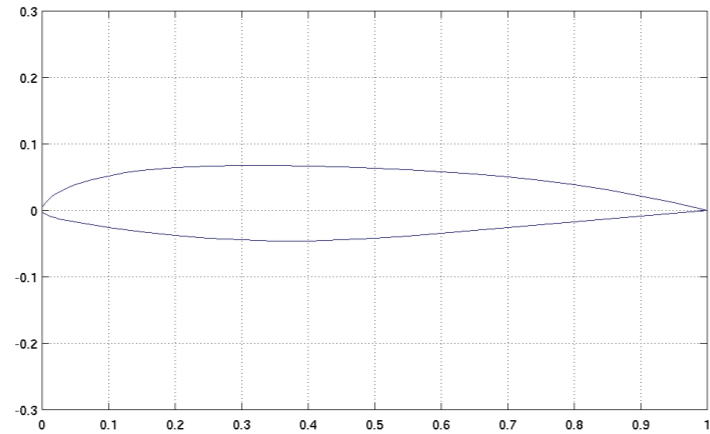
BOEING BACXXX AIRFOIL
