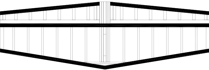
W1 Thru W 11 RIB Layout (typical) 3 SHEETS 1/8 x 3 Balsa
